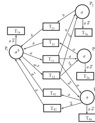
Fig. 2. CPL-net equivalent to II
